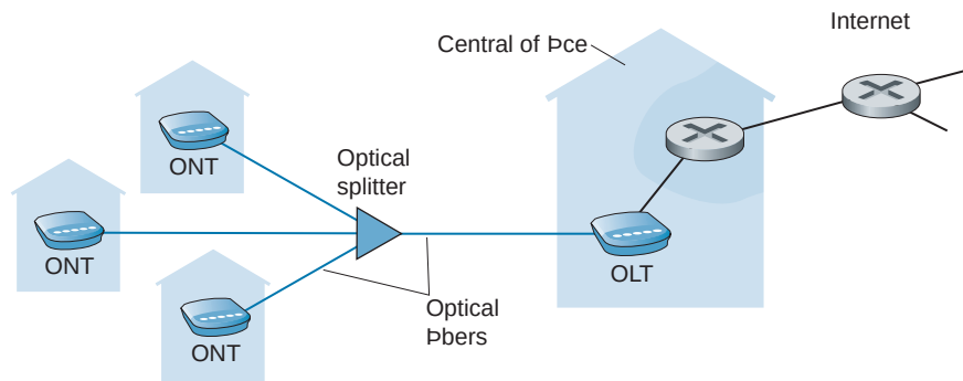
Figure 1.7 ♦ FTTH Internet access
